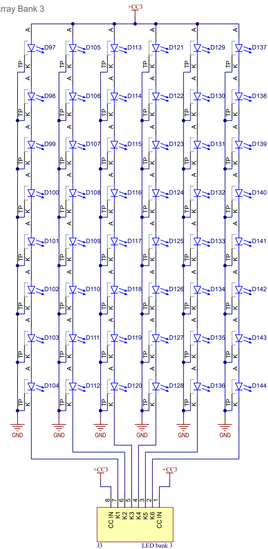
LED Array Bank 3
