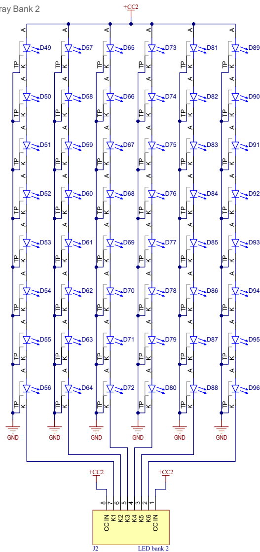
LED Array Bank 2
